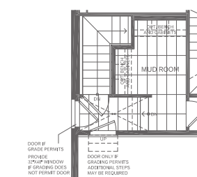
Opt. Mudroom Ground Floor
